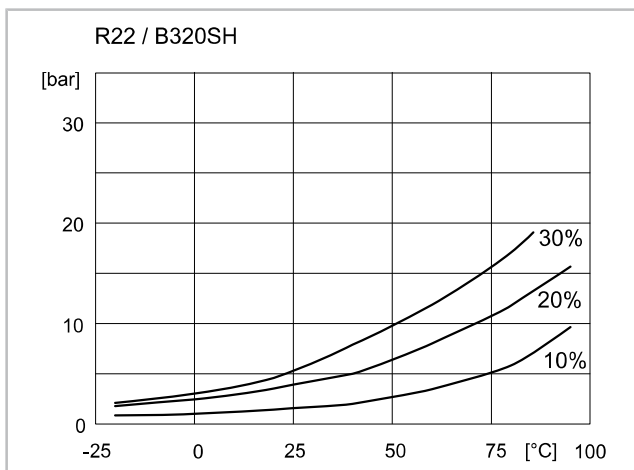
Fig. 10: Oil B320SH: Refrigerant pressure depending on oil temperature and refrigerant content (mass % of refrigerant in oil-refrigerant blend).
