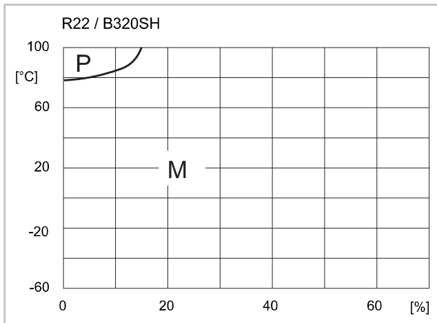
Fig. 9: Miscibility gaps for oil B320SH: Limit temperature depending on oil content (mass % of oil in oil refrigerant blend).
